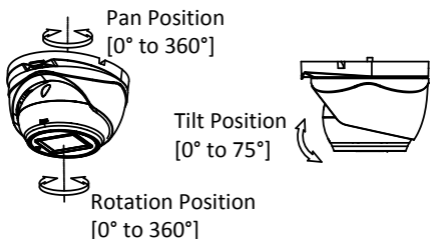
Figure 2-11 3-axis Adjustment
