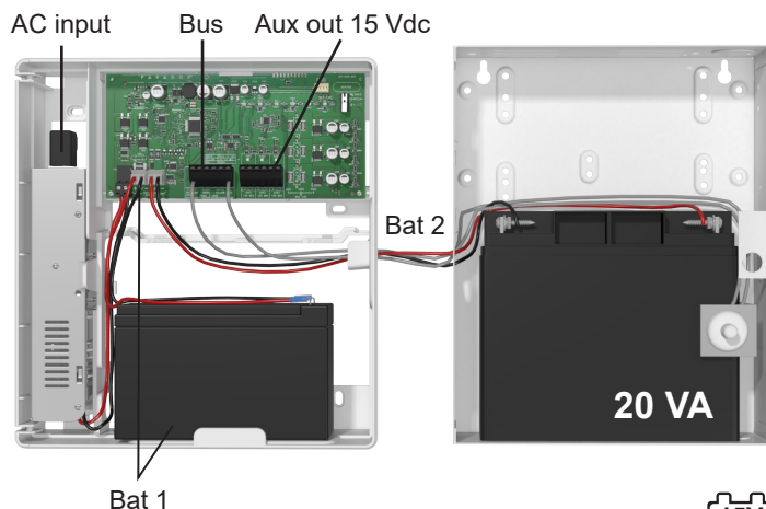
PS45 dual box installation
