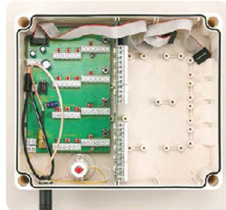
EXPANSION MODULE INSTALLED IN RECEIVER ENCLOSURE
