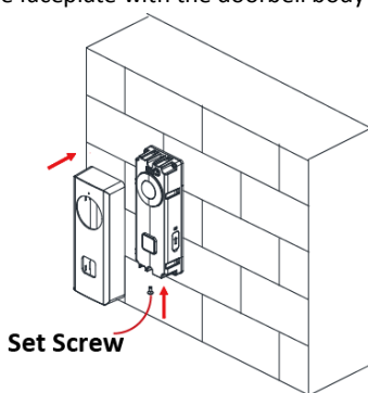
Figure 2-8 Fix Doorbell
