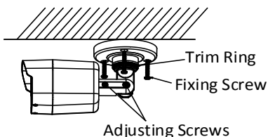
Figure 2-2 Fix the Camera to the Ceiling
