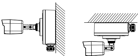
Figure 2-6 Fix the Camera to the Ceiling/Wall
