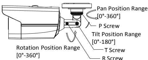
Figure 2-9 3-axis Adjustment
