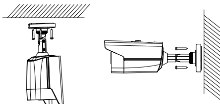
Figure 2-8 Fix the Camera to the Ceiling/Wall
