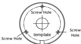
Figure 2-1 Drill Template
