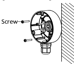
Figure 2-12 Fix the Camera to the Ceiling
