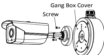
Figure 2-11 Fix the Camera with the Gang Box
