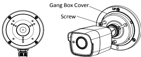
Figure 2-4 Fix the Camera with the Gang Box
