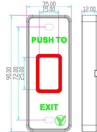
TSK-830NA(LED)
