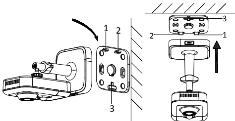
Figure 3-11 Buckle the Camera into Adapter Plate
