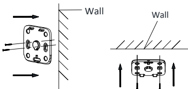
Figure 3-10 Install the Adapter Plate
